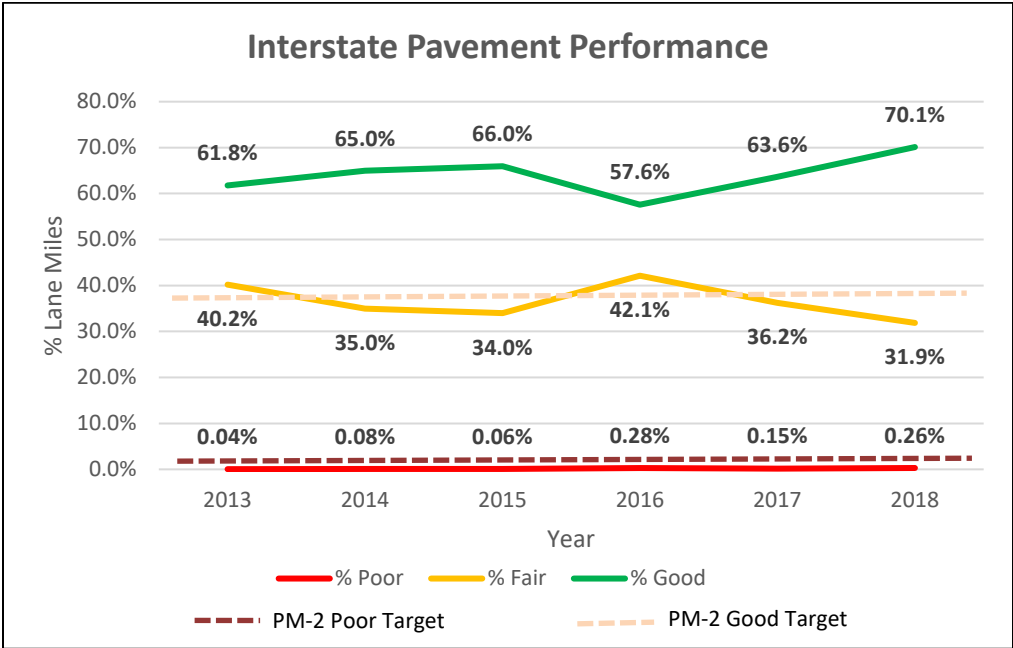
Figure 3-1: NHS Interstate Pavement Performance (MAP-21 Measures)
